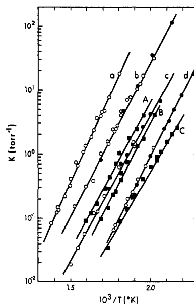
Figure 4. van't Hoff plots of equilibrium constants for reactions B_1H^+ + B_2 = B_1H^+B_2 : ( B_1, B_2 ): (a) NH_3, NH_3 ; (b) CH_3NH_2, CH_3NH_2 ; (c) (CH_3)_2NH, (CH_3)_2NH ; (d) (CH_3)_3N, (CH_3)_3N ; (A) CH_3NH_2, NH_3 ; (B) (CH_3)_2NH, CH_3NH_2 ; (C) (CH_3)_3N, (CH_3)_2N . (○) B_1 = B_2 , total pressure due to amine only. (●) B_1 = B_2 , major gas CH_4 .
