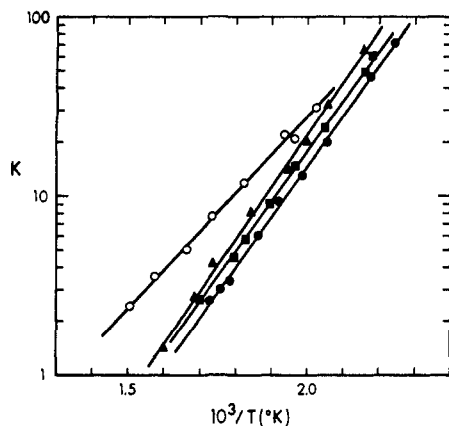
Figure 5. van't Hoff plots of proton transfer reactions B_1H^+ + B_2 = B_1 + B_2H^+ where B_1 is a monoamine and B_2 an \alpha,\omega -diamine capable of proton induced cyclization: (○) dimethylamine, 1,2-diaminoethane; (●) trimethylamine, 1,3-diaminopropane; (▲) trimethylamine, 1,5-diaminopentane; (■) trimethylamine, 1,7-diaminoheptane.
